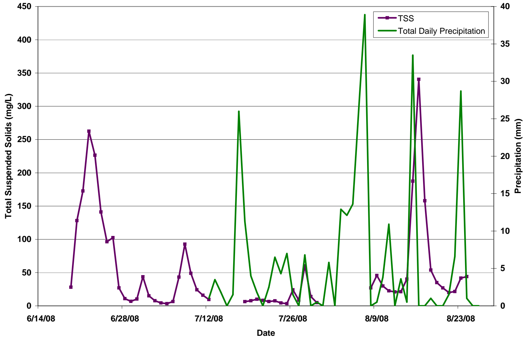
Total Suspended Solids and Precipitation at Duncan Creek 2008
